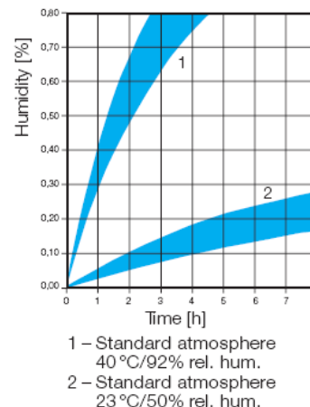
Moisture absorption Polyether-TPU Hardness 80 Shore A – 64 Shore D
